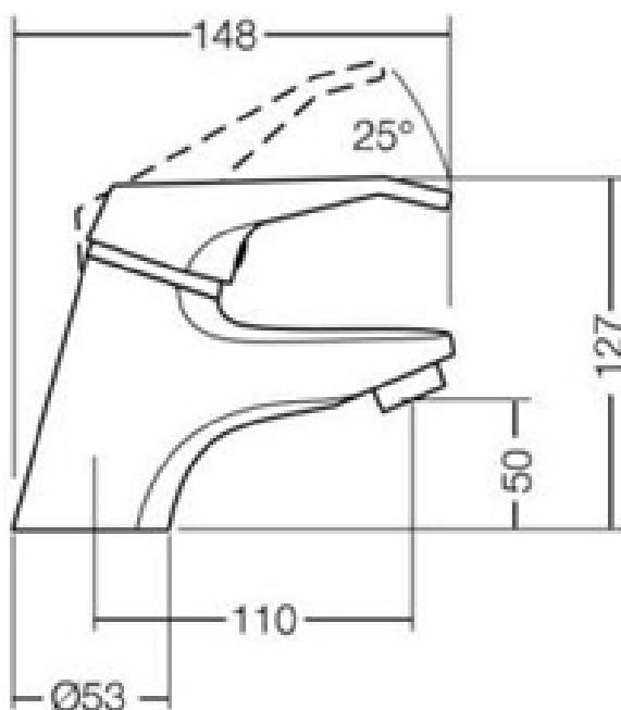
TECHNICAL DRAWING
